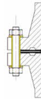
Tipo VCS Ring Joint
